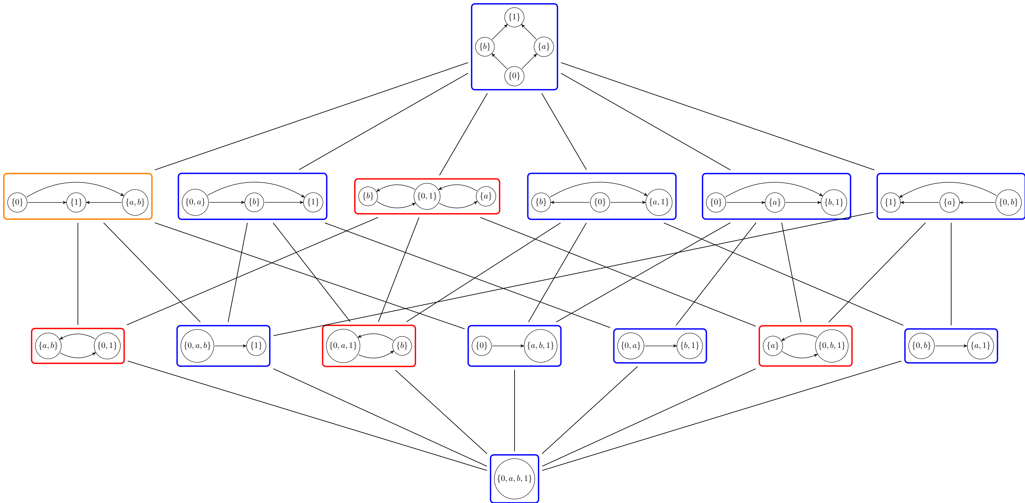
Faces of the Order Polytope \mathcal{O}(E) are in bijection with the (closed) E -connected, E -compatible partitions (in blue)
